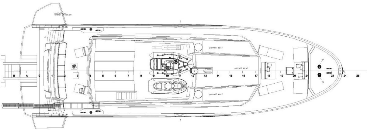
Upper level
