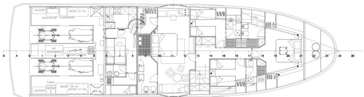
Lower deck
