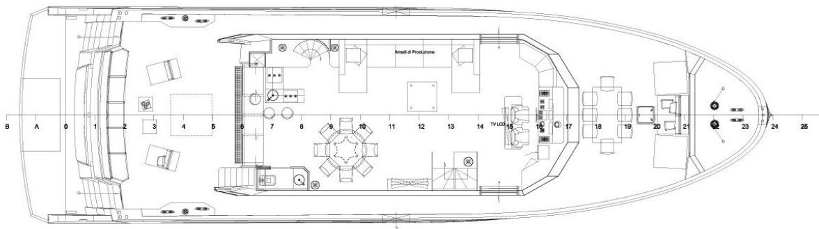
Main deck
